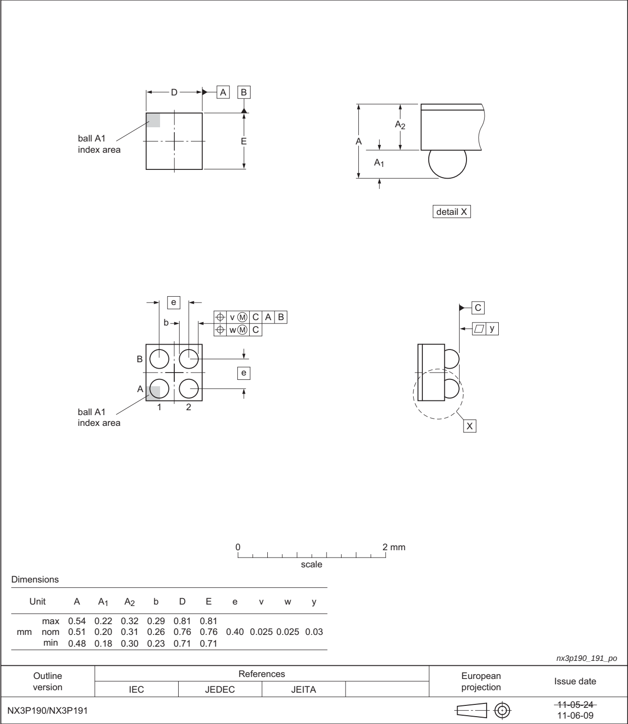
Fig 18. Package outline WLCSP4 (NX3P190/NX3P191)
